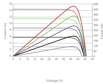
Current-Voltage & Power-Voltage Curves (575W)
